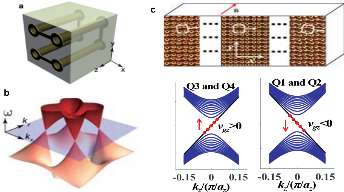
Metamaterials hosting ideal Weyl points in the momentum space. a. the unit cell of the ideal Weyl metamaterial formed by saddle-shaped metallic loop. b. The band structure of metamaterial shows that there are four ideal points located at the same frequency, as protected by the symmetry of the unit cell. c. By introducing inhomogeneity to the ideal Weyl metamaterial, an effective magnetic field can be induced, which leads to formation of chiral zero modes, which are one-way propagating bulk modes.
